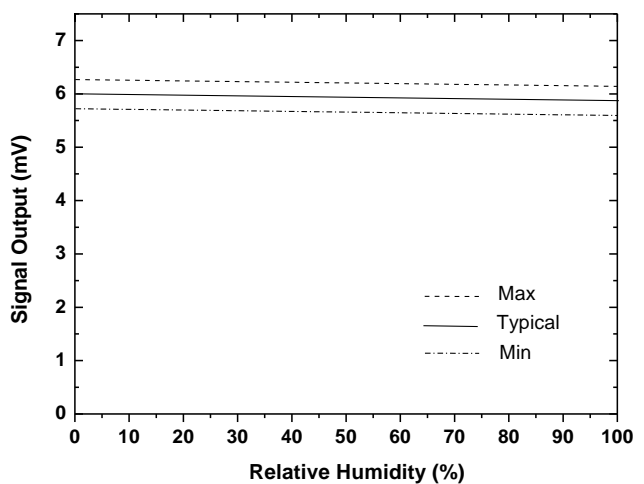
Fig 5. Humidity dependency
